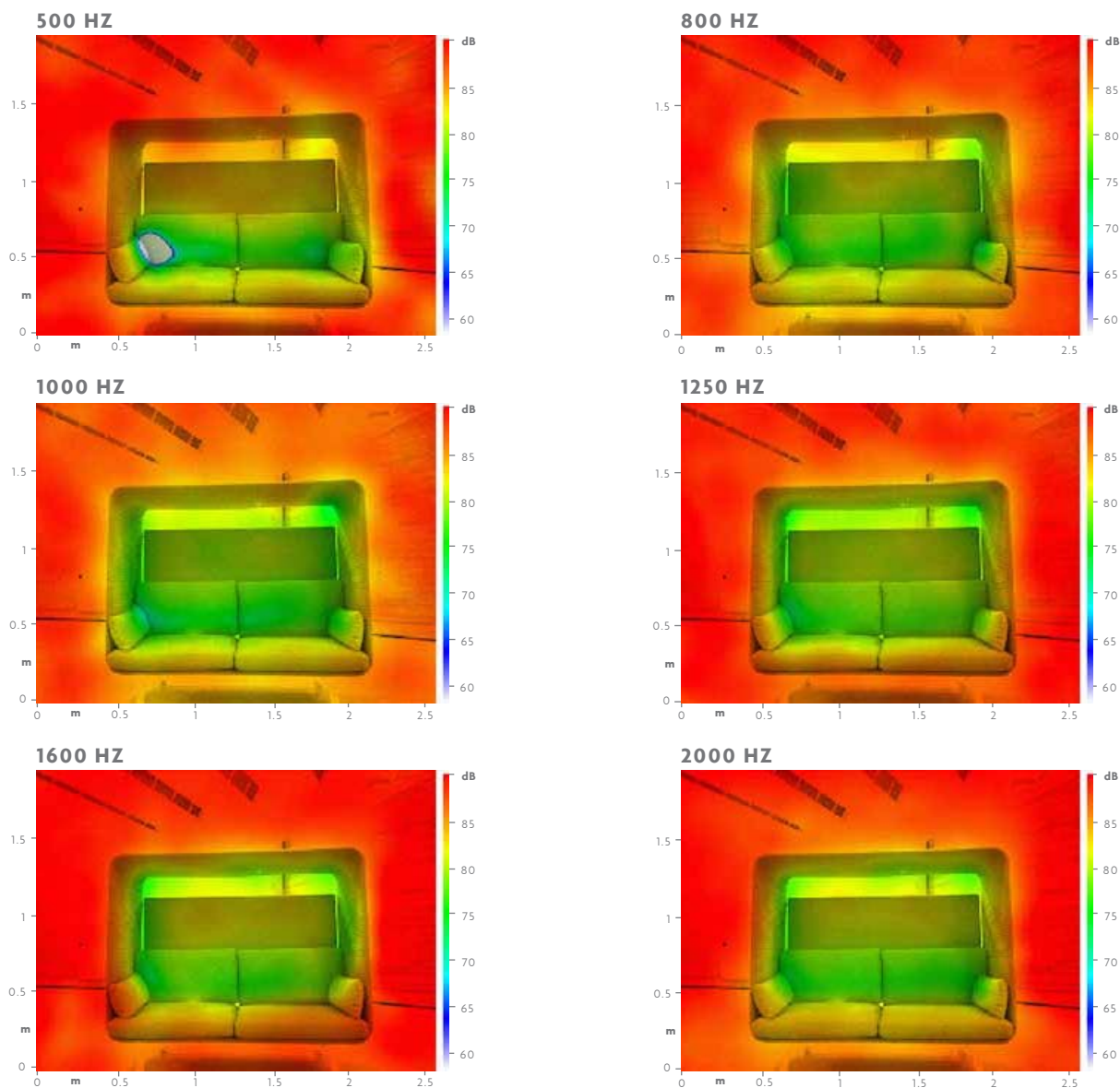
Sound Intensity Test conducted on 20/01/2014 at Z Lab S.r.l. Cerea (VR)
